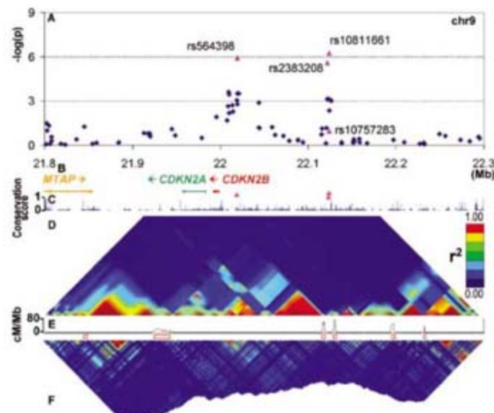
conservation. (D) GoldSurfer2 (25) plot of linkage disequilibrium ( r^2 ) for SNPs genotyped in WTCCC scan (passing T2D-specific quality control) in WTCCC T2D cases. (E) Recombination rate given as cM/Mb. Red boxes represent recombination hotspots (26). (F) GoldSurfer2 plot of linkage disequilibrium ( r^2 ) for all HapMap (haplotype map of the human genome) SNPs across the region (HapMap CEU data) (27). Fig. 2. (right) Overview of chr9 signal region. Panel layout as in Fig. 1.
